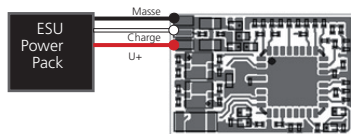
Figure 2: Connection to LokPilot DCC with Next 18 connector
